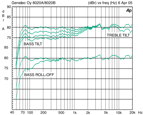
Figure 4. The curves show the effect of the “Bass Tilt”, “Treble Tilt” and “Bass Roll-Off” controls on the free field response of the 8020B
