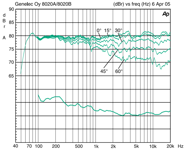
Figure 5. The upper curve group shows the horizontal directivity characteristics of the 8020B measured at 1 m. The lower curve shows the system's power response.
